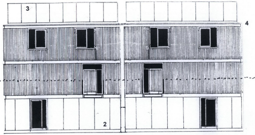
SOUTH EAST (STREET) ELEVATION
