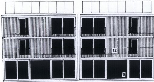
NORTH WEST (GARDEN) ELEVATION
